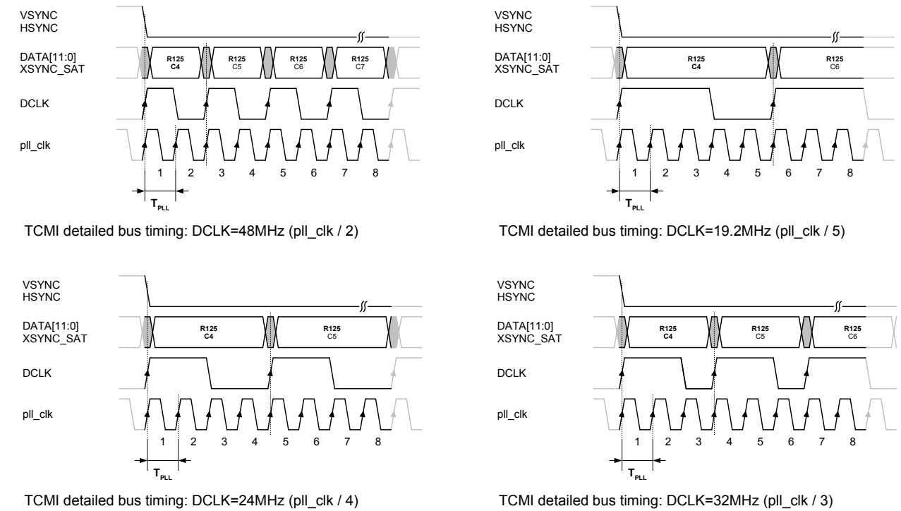
Figure 28: TCMI timing examples with symmetric and asymmetric DCLK
