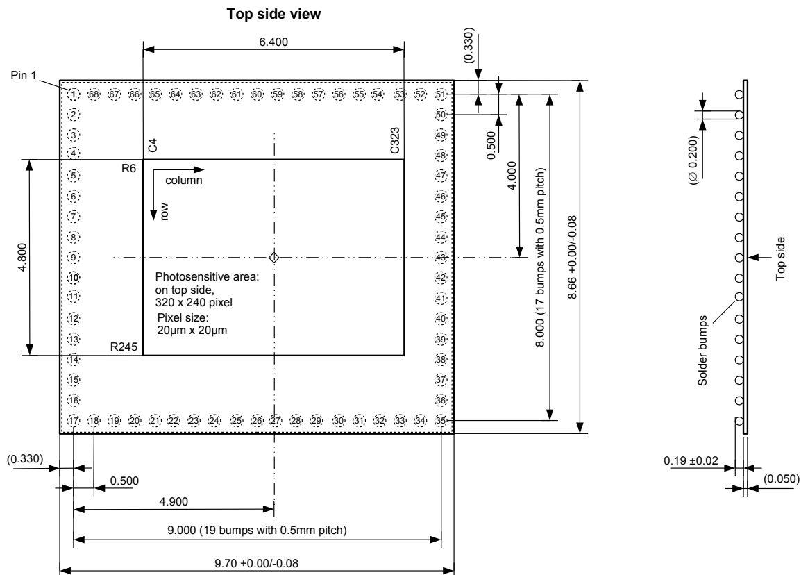
Figure 10: Mechanical dimensions
