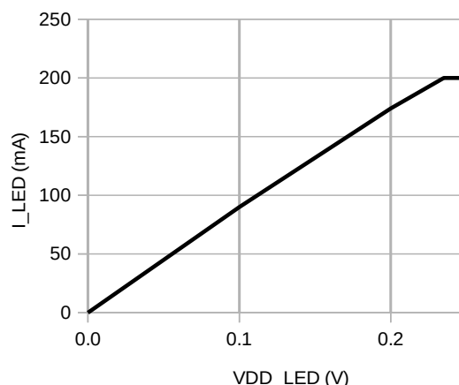
Figure 18: Output characteristic I_{LED} versus V_{DDLED} . Refer for maximum values of V_{DDLED} and I_{LED} to Table 1 and Table 2
