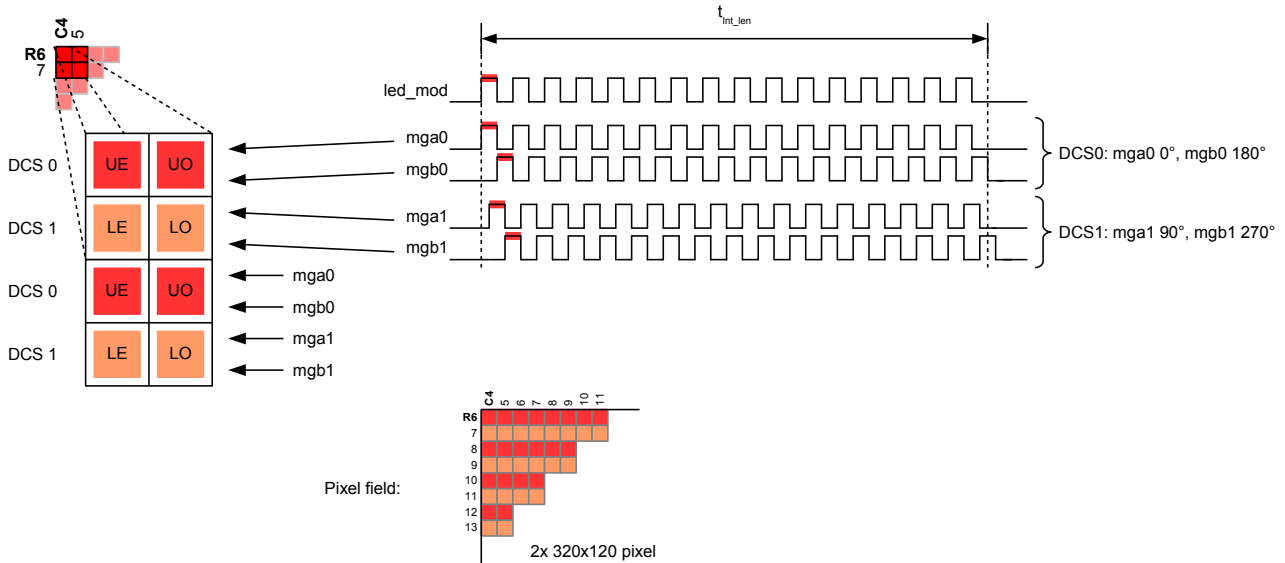
Figure 39: Dual phase mode with phase-shifted integration time: even and odd rows independently controlled by mgx0 and mgx1 with different phase shifts
