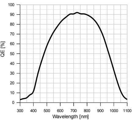
Figure 6: Typical quantum efficiency
