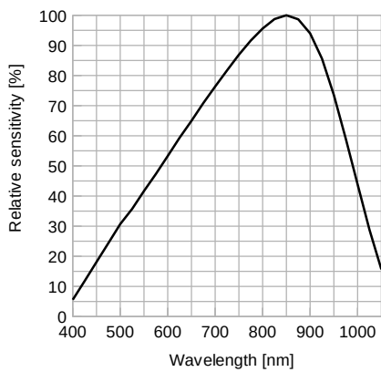
Figure 3: Relative spectral sensitivity ( S_{\lambda} ) vs. wavelength
