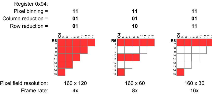
Figure 45: Row reduction on y-axis combined with horizontal and vertical binning
