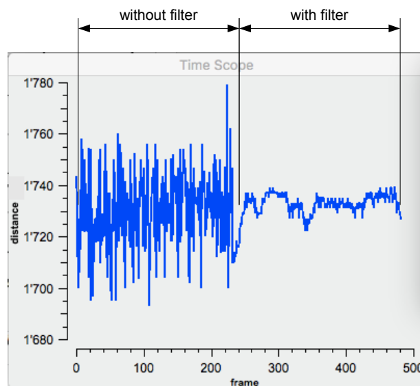
Figure 1: Distance noise reduction with the static Kalman filter on right section of the diagram (Distance in mm; amplitude at 200LSB)
